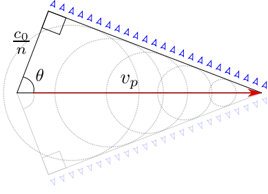
Figure 2: The angle at which Cherenkov radiation will be emitted at each unit distance. Note that the particle in this figure is significantly faster than the other ones to better illustrate the concept.
